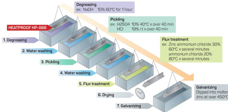
Example of hot dip galvanizing process
